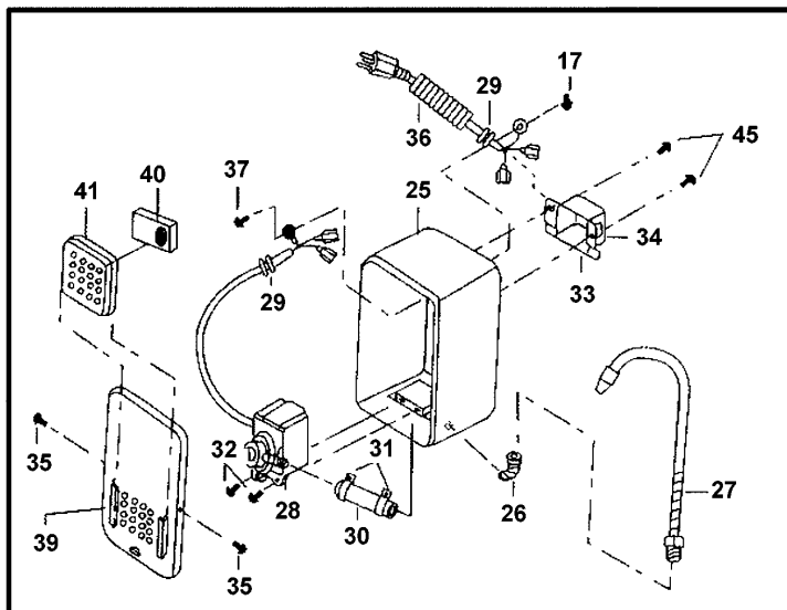
Exploded view of the pump assembly
